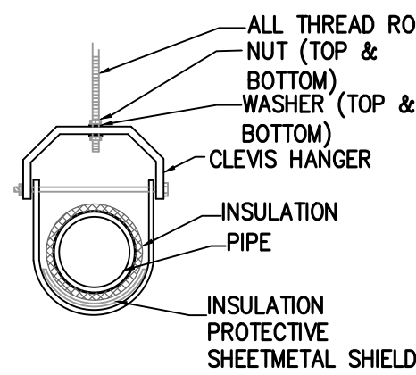
TYPICAL CLEVIS HANGER DETAIL
