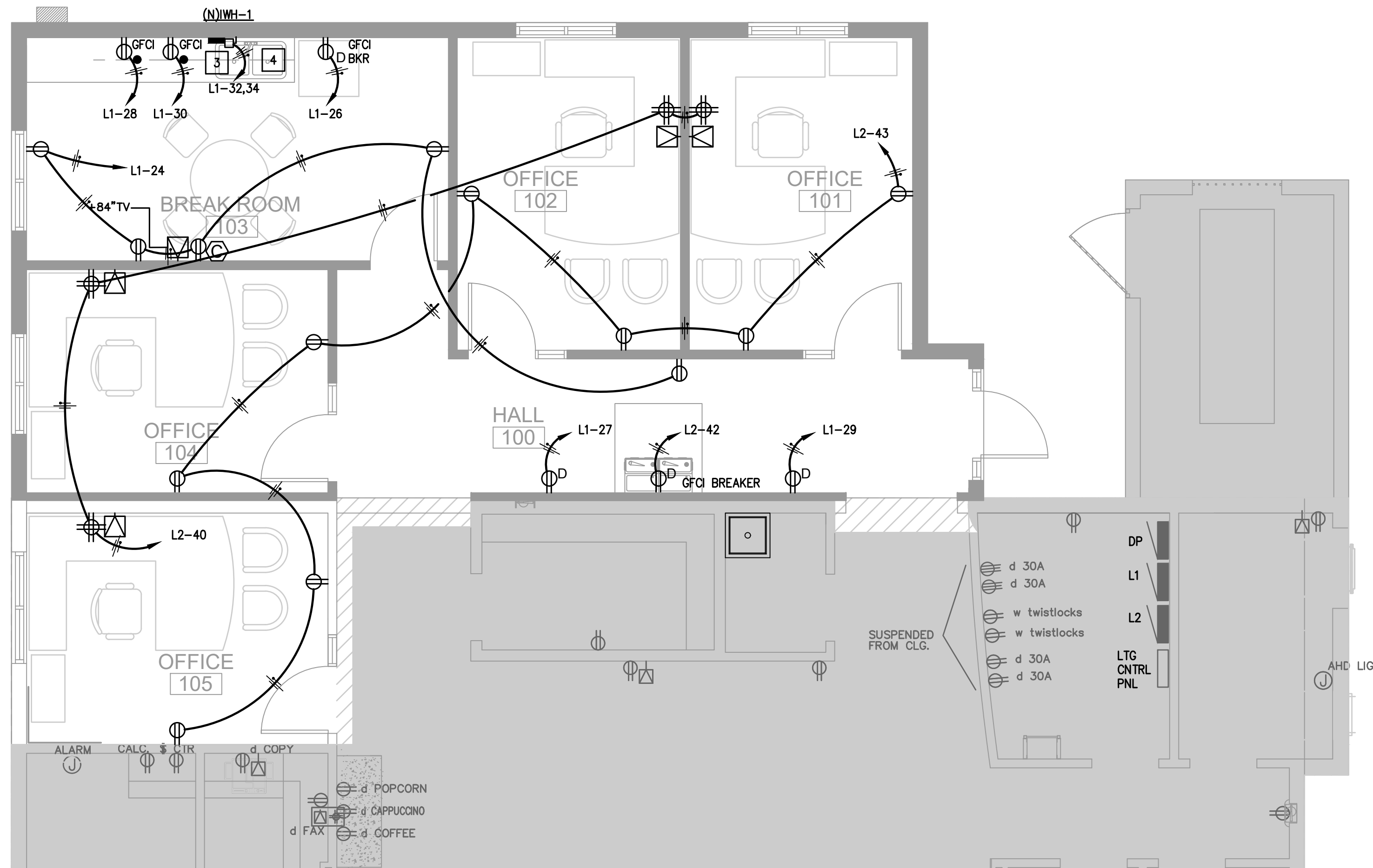
01 ELECTRICAL POWER PLAN SCALE: 1/4"=1'-0"
