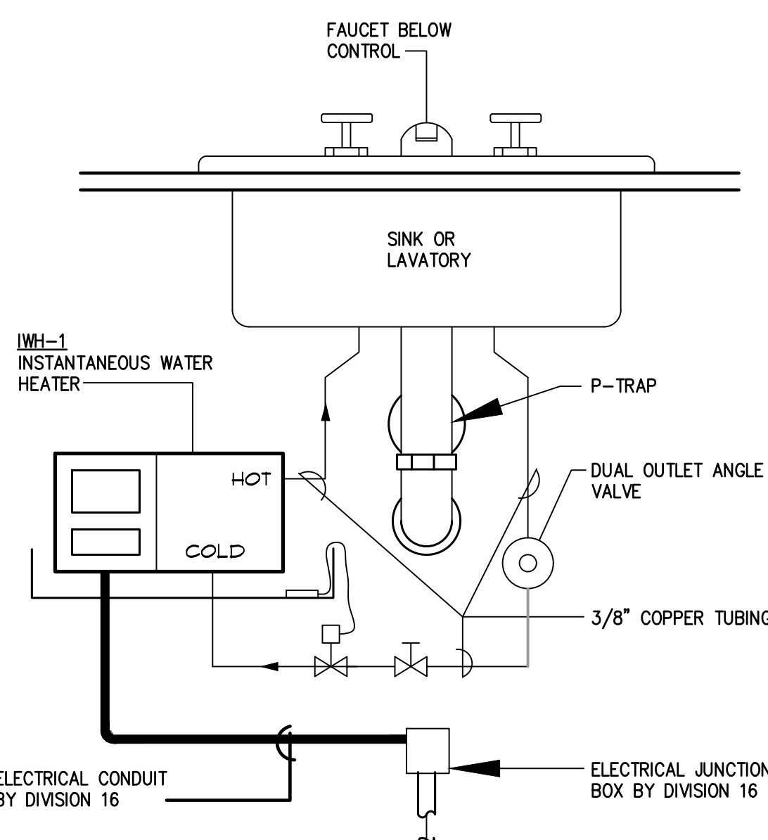
03 INSTANTANEOUS WATER HEATER DET. SCALE: NONE
