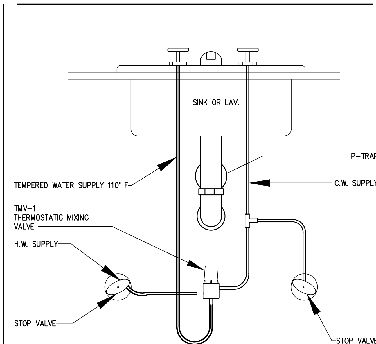
02 THERMOSTATIC MIXING VALVE TMV-1 SCALE: NONE
